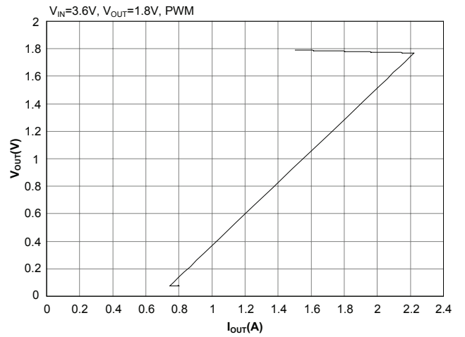
Current Limit
